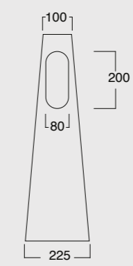
Cod. 3500101 Colonna Equilibrium scarico parete Column Equilibrium wall drain
